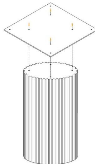
IMAGE 3 - Metal bridge plate assembly with base
